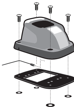
Charging Station with Embedded CodeXML® Modem
